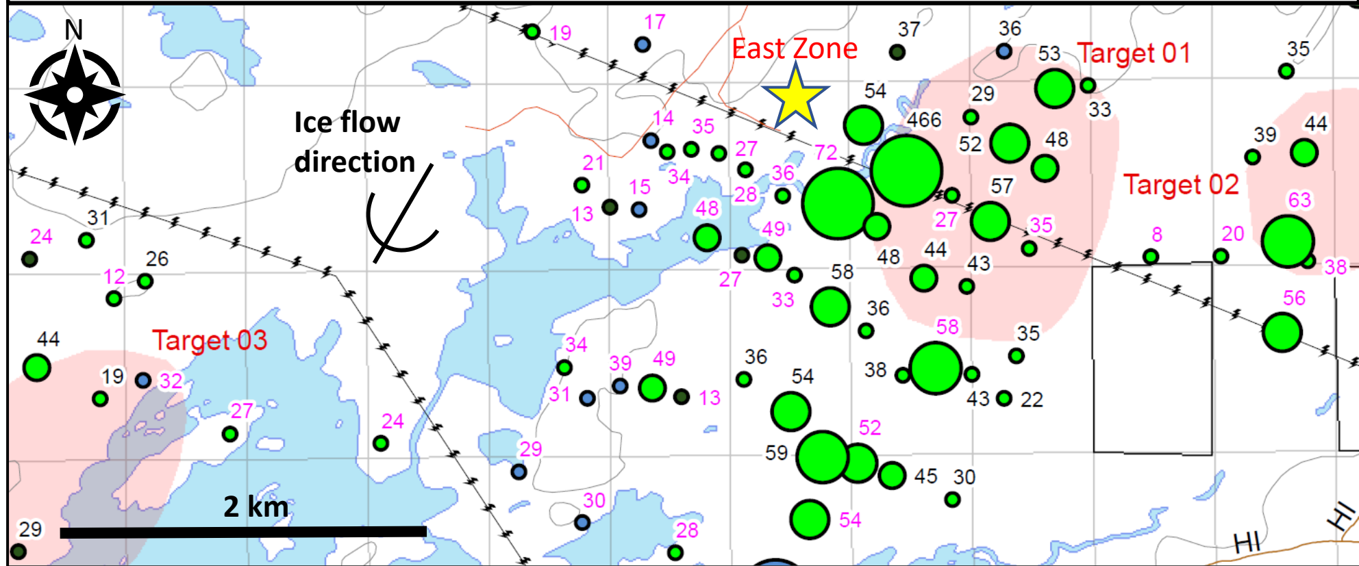
Map 2 – Detail of Till Sampling Results Target #1,2,3 Areas - Gold Grain Count Normalized to 10 kg
